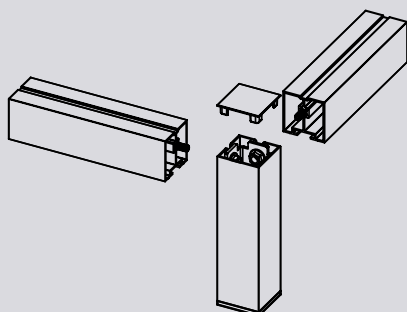
Aggancio piede terminale End leg's fixing
