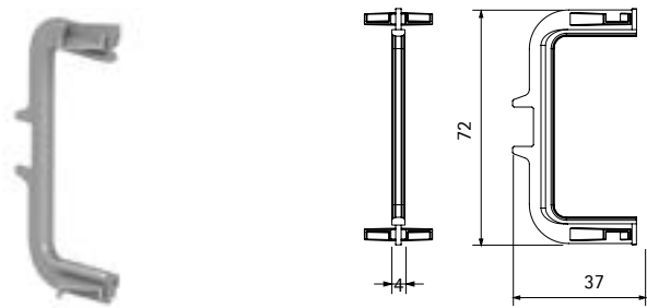
Angolo interno 90° G13 in plastica Plastic 90° internal corner for G13
