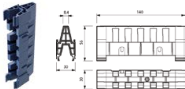
Easy lock Accessorio per clap'n fit Accessory for clap'n'fit
