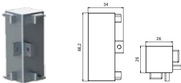
Angolo in alluminio esterno cassetto External aluminum corner for drawer profile
