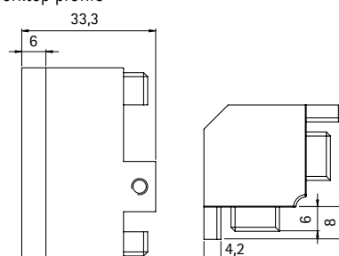
Angolo in alluminio interno sottotop Internal aluminum corner for worktop profile
