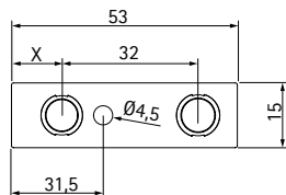
X da 7,5 a 20mm X from 7,5 to 20mm
